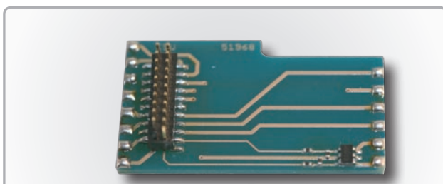
21MTC adapter board 2
