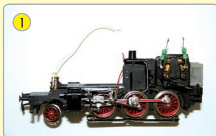
1 After adding the permanent magnet to the motor of your Delta® loco (as shown on the left page), remove the old Delta® decoder.
