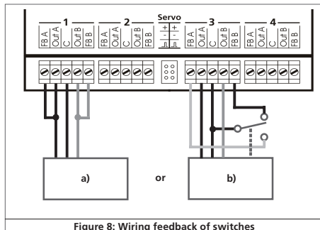
Figure 8: Wiring feedback of switches
