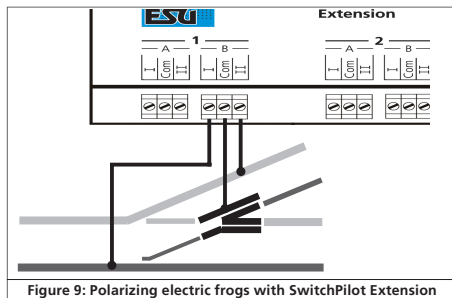
Figure 9: Polarizing electric frogs with SwitchPilot Extension
