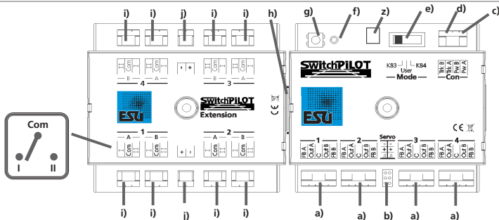
Figure 1: SwitchPilot connected with SwitchPilot Extension
